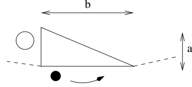
Fig. 8. A worst case navigation example. If b \gg a , and if the robot chooses to follow the gap on the right, practically the whole triangle boundary will be followed to reach the circle.
