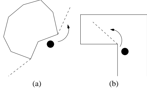
Fig. 6. Not all gaps disappear when chased. If the obstacles in which the gap begins and ends are different, the gap does not disappear (a). The gaps disappears if the gap begins and ends in the same obstacle (b).
