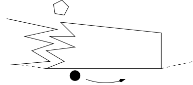
Fig. 9. Paths with shortest gaps sequence are preferred. The robot will follow the path on the right, because it offers less gaps to chase, although is not the shortest path. With only gaps information, the robot cannot do better.
